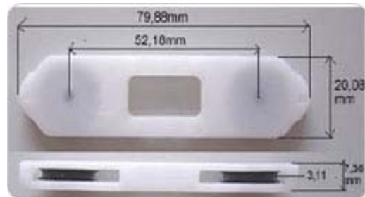
P1: PULLEY MULLER MJ2 BIG
